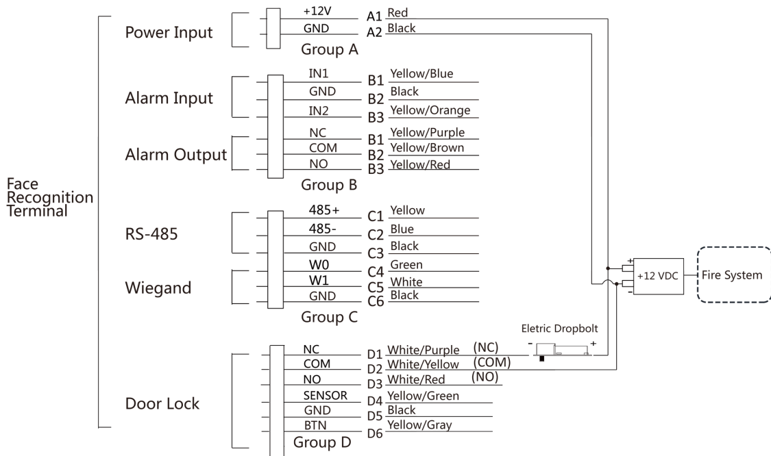
Figure 4-4 Wire Device
