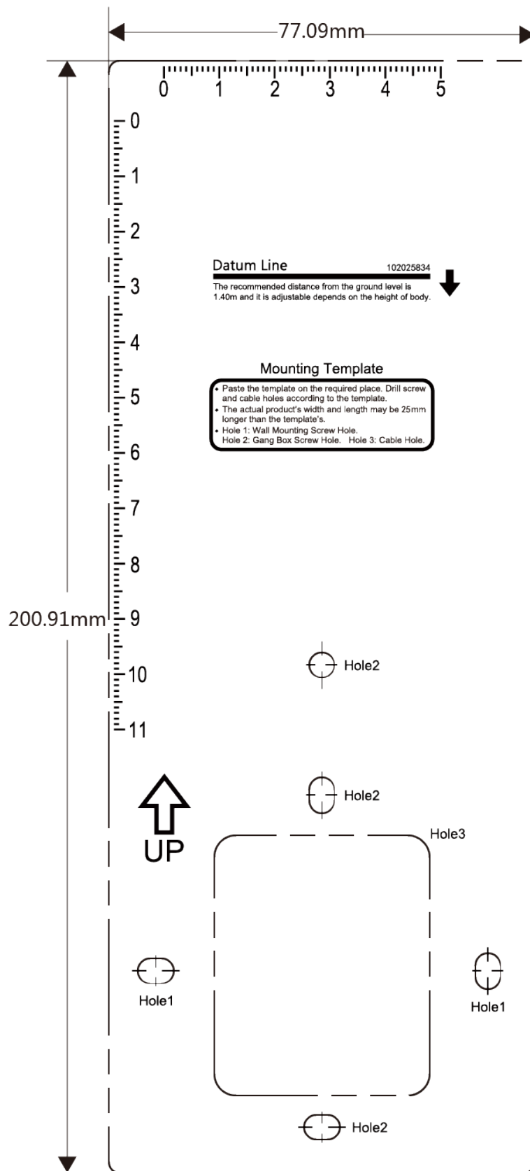
Figure 3-1 Mounting Template
