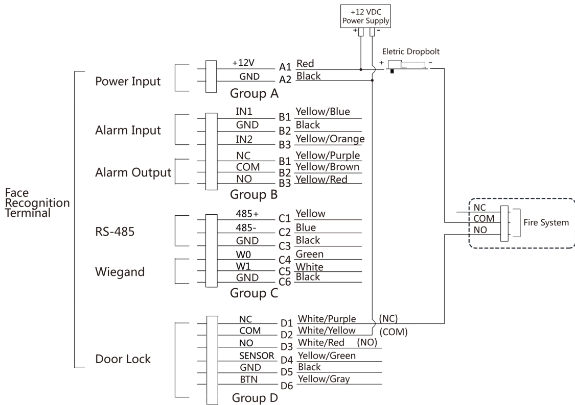
Figure 4-6 Wiring Device
