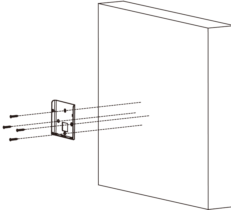
Figure 3-2 Install Mounting Plate
