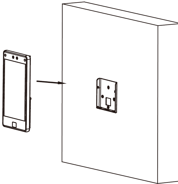
Figure 3-3 Hang Device
