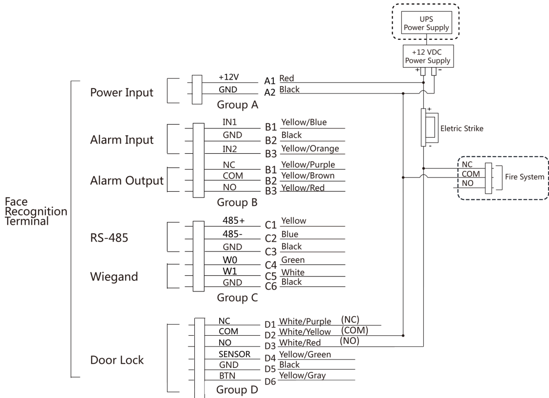
Figure 4-8 Device Wiring
