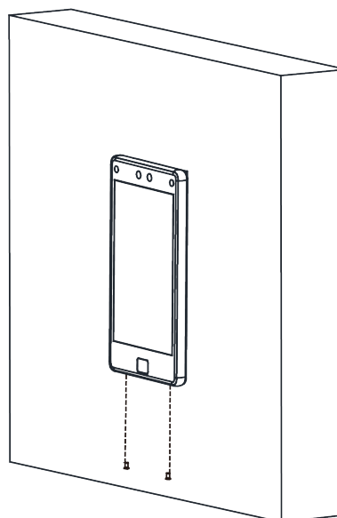
Figure 3-4 Secure Device
