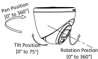
Figure 2-9 3-Axis Adjustment
