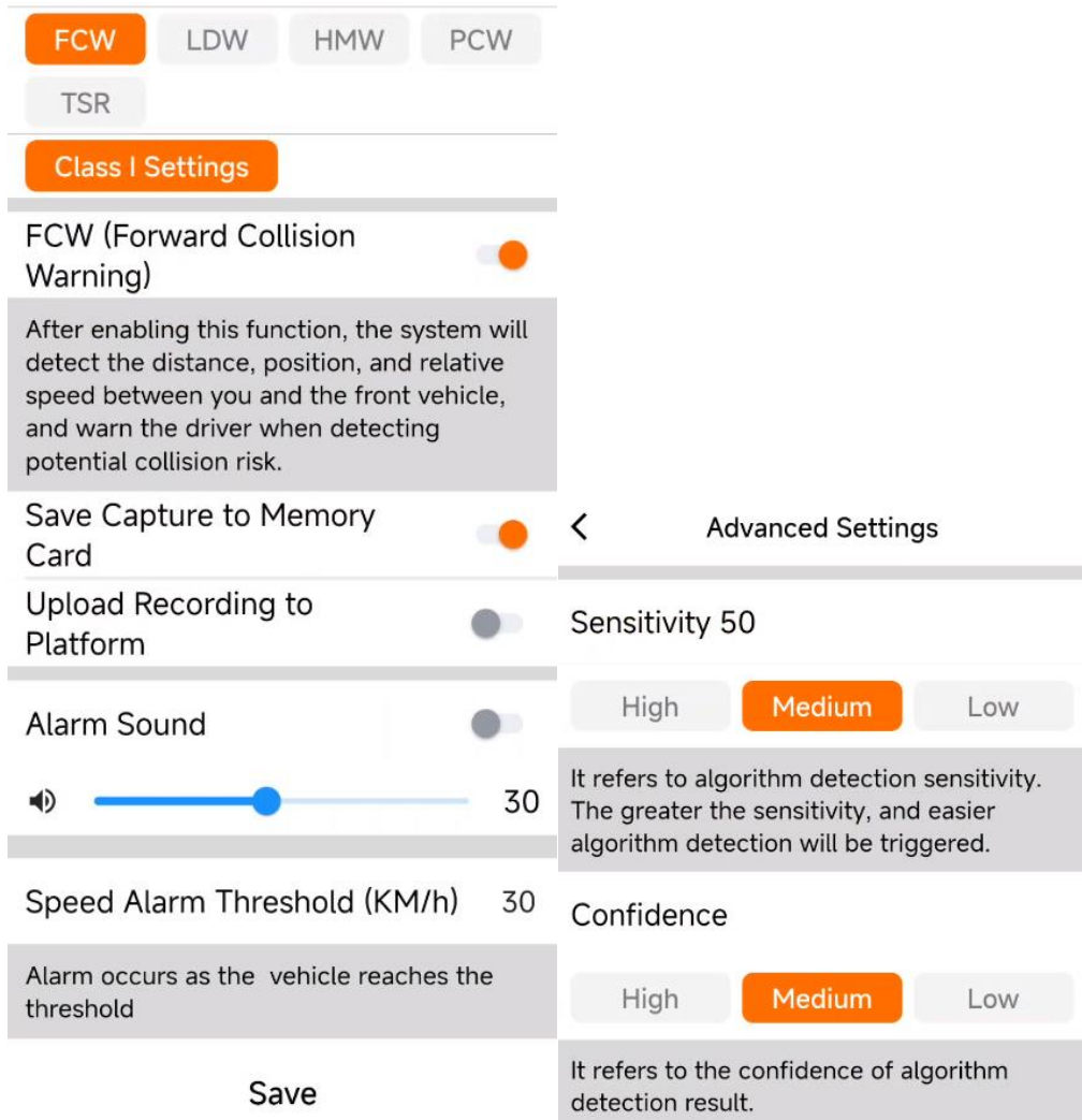
Figure 15-6 ADAS Parameter Settings and Advanced Settings
